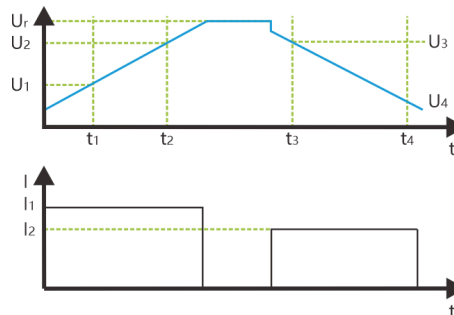
▲ Capacitance Calculation Graph
