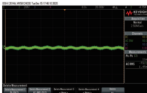
▲ Ripple Waveform
